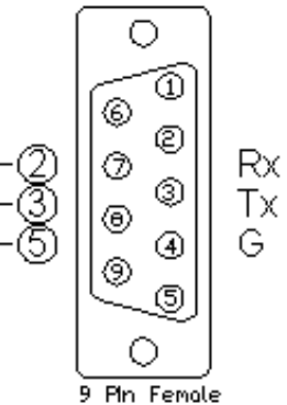
Rear View of Connector
